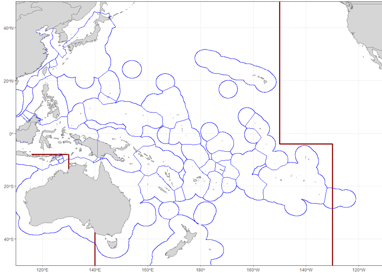
Figure 3. Approximate 200-mile zones in the WCPFC Statistical Area
