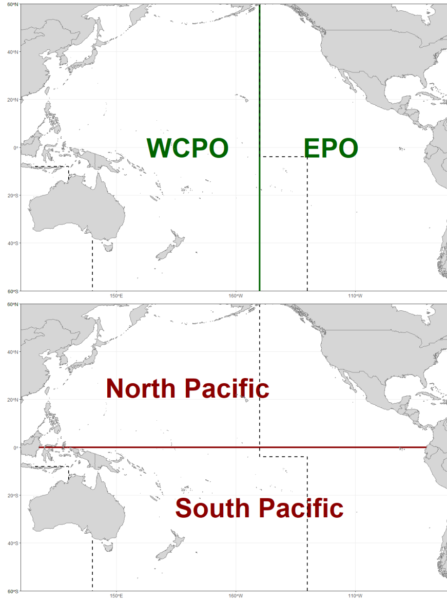
Figure 2. Western and Central Pacific Ocean (WCPO) / Eastern Pacific Ocean (EPO), and the North / South Pacific Ocean
