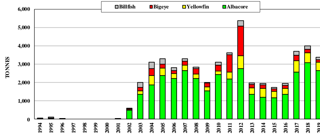
Figure 7. Catches by Cook Islands longliners
