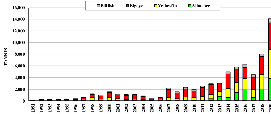
Figure 8. Catches by Federated States of Micronesia longliners
