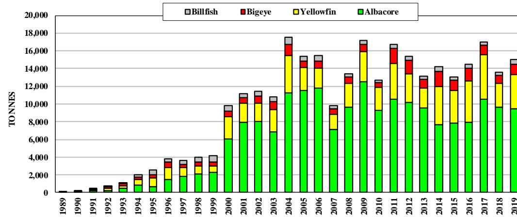
Figure 9. Catches by Fiji Islands longliners
